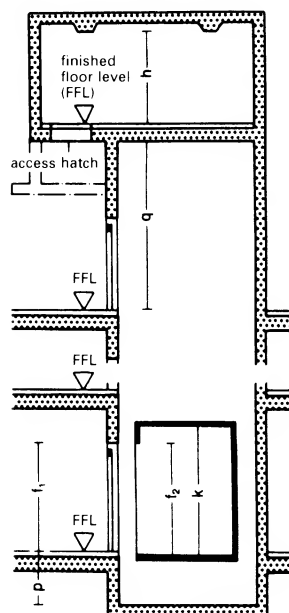
3 Lift motor room
